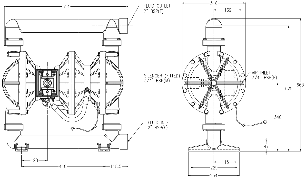
B50 / X50 General Assembly :- All dimensions +/- 3mm
